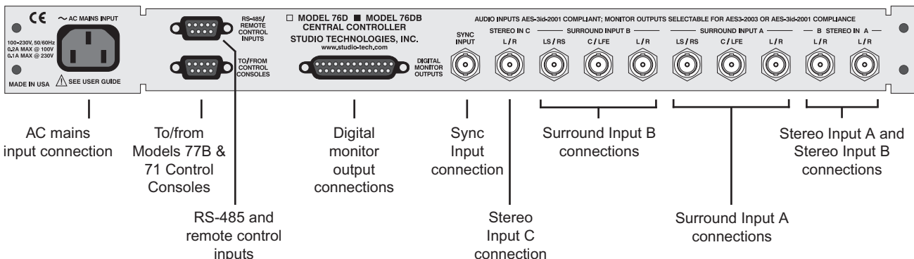
Figure 2. Model 76DB Central Controller Back Panel
