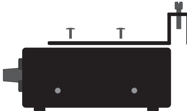
Attach adapter to the Model 35 Talent Amplifier as shown.
