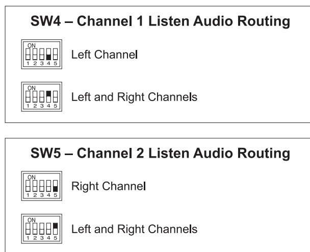
Figure 5. Channel 1 and channel 2 headphone audio routing mode configuration switches
