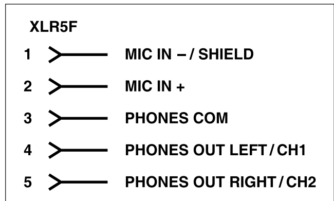
Figure 2. Headset connection pinout chart
