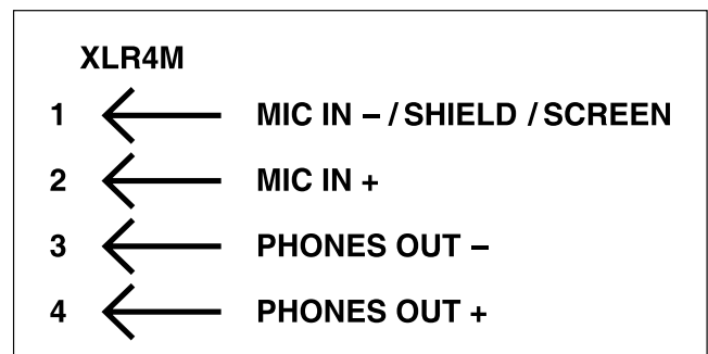
Figure 2. Headset connection pinout chart
