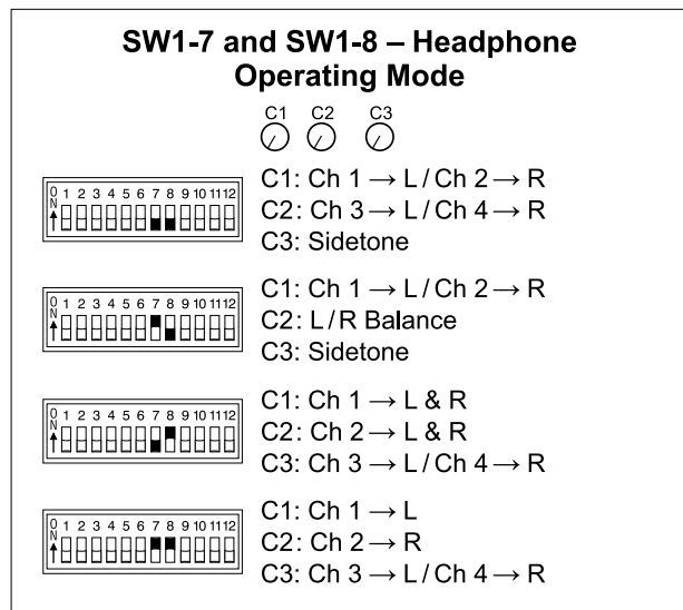
Figure 7. Headphone operating mode switch settings
