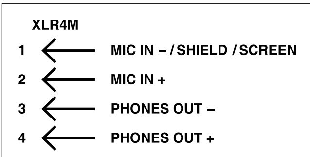
Figure 2. Headset A connection pinout chart
