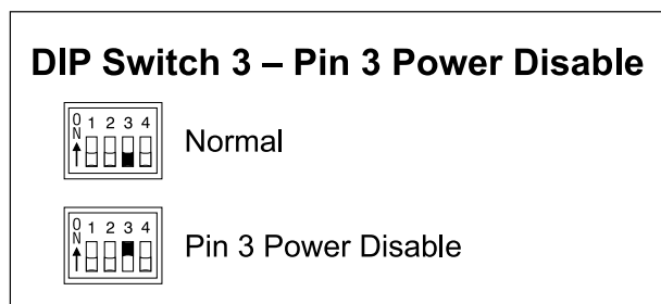
Figure 9. DIP Switch 3—Pin 3 Power Disable
