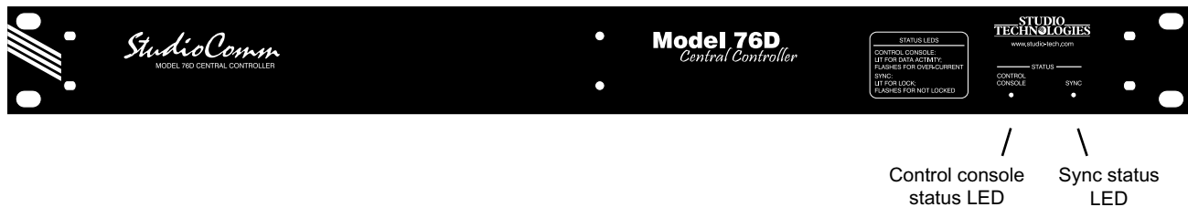
Figure 1. Model 76D Central Controller Front Panel
