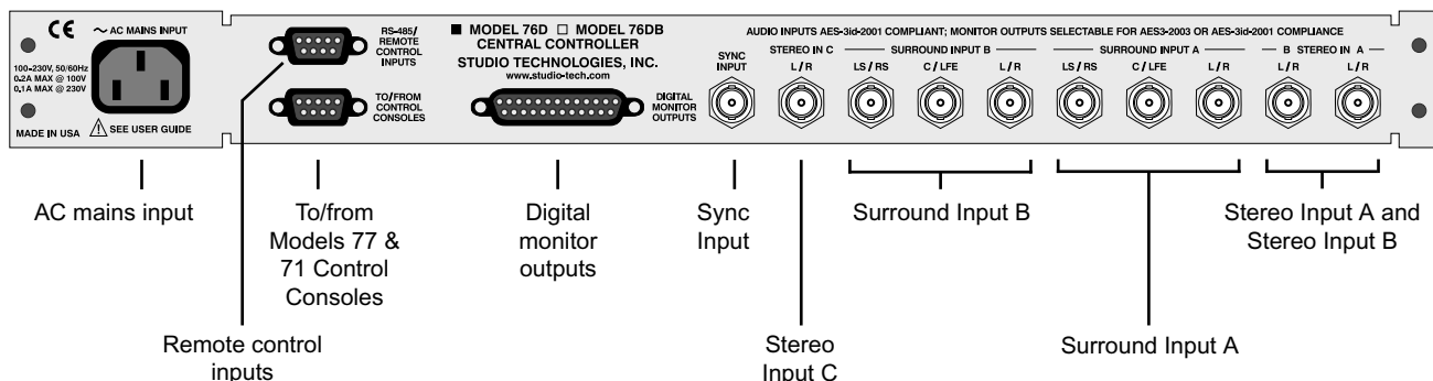
Figure 2. Model 76D Central Controller Back Panel
