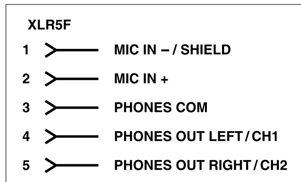
Figure 2. Headset connection pinout chart
