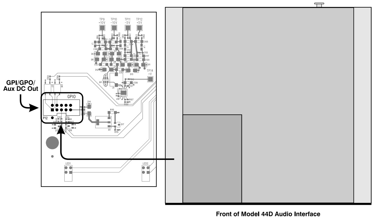
Figure 10. Model 44D GPI/GPO/Aux DC Out 10-pin header location (applies to M44D-00151-00250)
