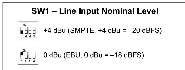
Figure 4. Analog inputs nominal level configuration switch
