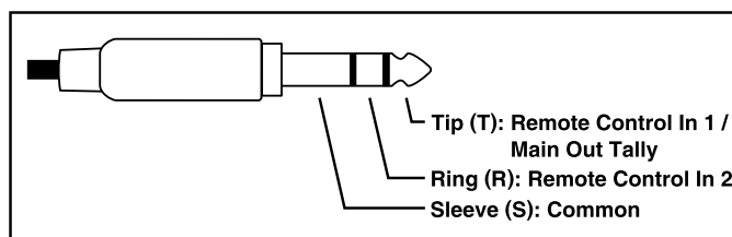
Figure 2. 3-conductor (TRS) 3.5 mm plug configured for use with remote control inputs
