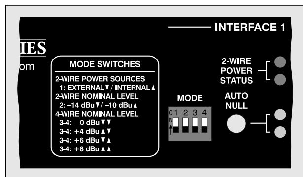
Figure 5. Detail of front panel showing four DIP switches
