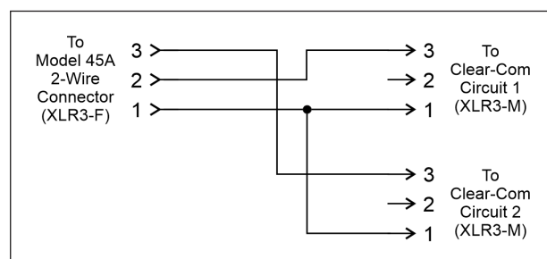
Figure 5. Adapter cable wiring diagram for Clear-Com single-channel party-line (PL) circuits
