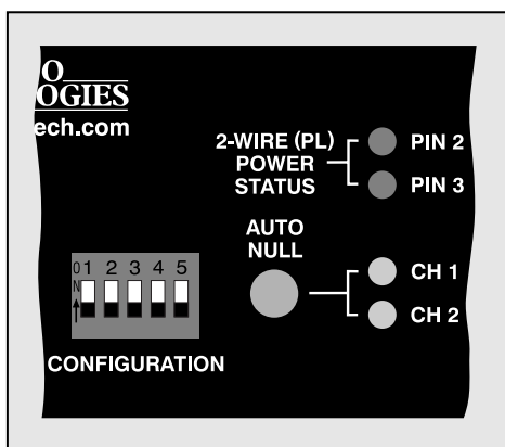
Figure 11. Detail of front panel showing auto null section
