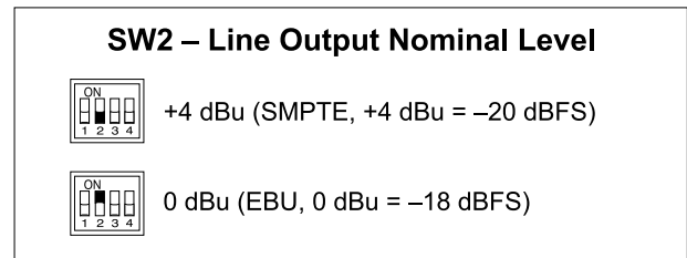
Figure 5. Analog outputs nominal level configuration switch
