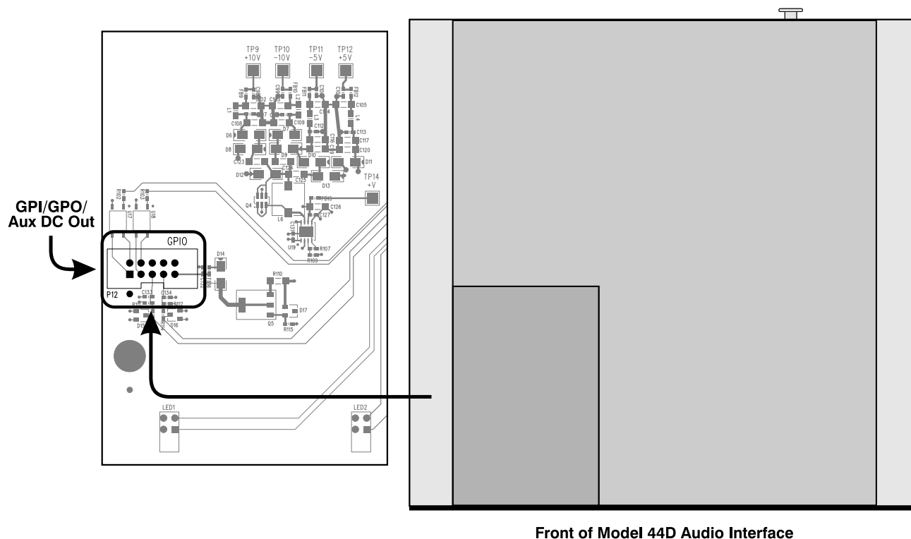
Figure 10. Model 44D GPI/GPO/Aux DC Out 10-pin header location (applies to M44D-00151-00250)
