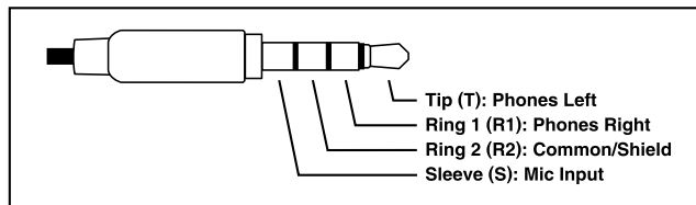
Figure 3. Headset B 4-conductor 3.5 mm TRRS connection pinout diagram
