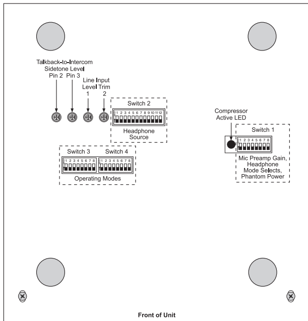
Intercom Pin 2 is RTS™ TW Channel 1. Intercom Pin 3 is RTS™ TW Channel 2, or Clear-Corr® Channel 1.
