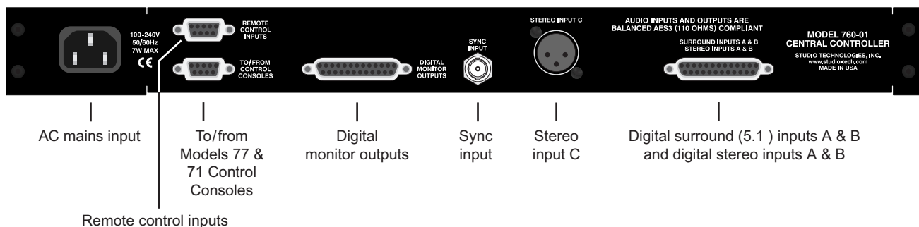
Figure 2. Model 760-01 Central Controller Back Panel
