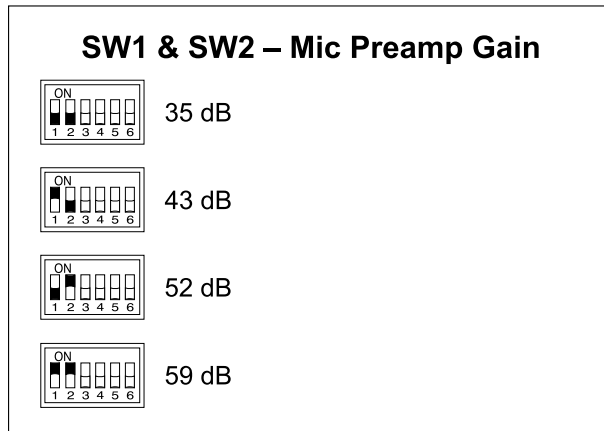
Figure 2. Microphone preamplifier gain configuration switches
