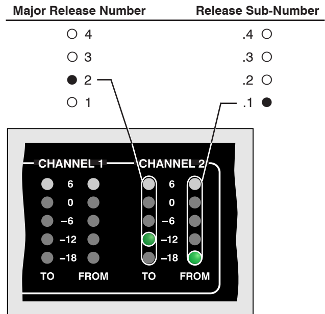
Figure 4. Detail of front panel showing the status LEDs that display the application firmware version. In this example, the application firmware version is 2.1.
